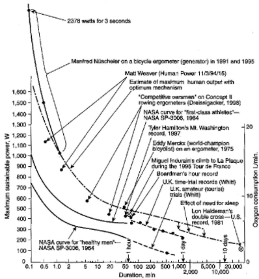
Figure 2.4 Human power output, principally by pedaling. Curves connect the terminations through exhaustion of constant-power tests. (Data collected by Dave Wilson added to an original NASA chart.)
