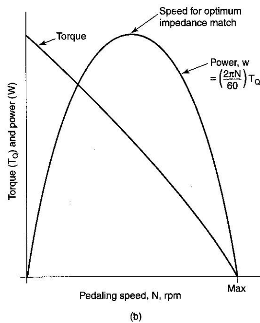
Figure 9.1 Impedance-match curve: (a) An ergometer used to develop a curve of maximum torque versus pedaling speed. (b) Torque and power versus pedaling speed, showing speed for optimum impedance match.
